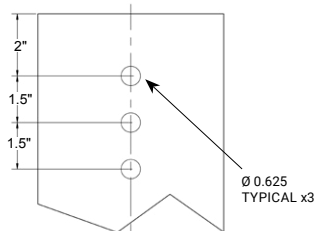
DRILL PATTERN
