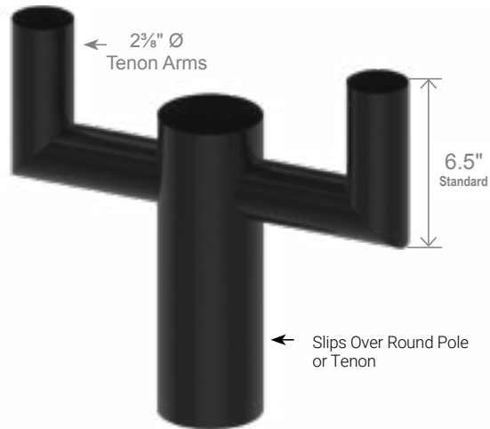
Bull Horn Pole Mounted Top (Double 180°)
